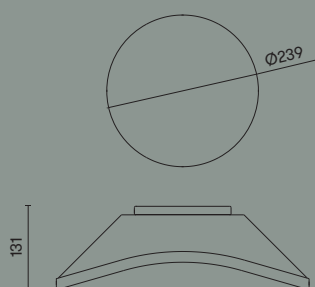
05-5276-BW-M1 (Mains dimming)*
