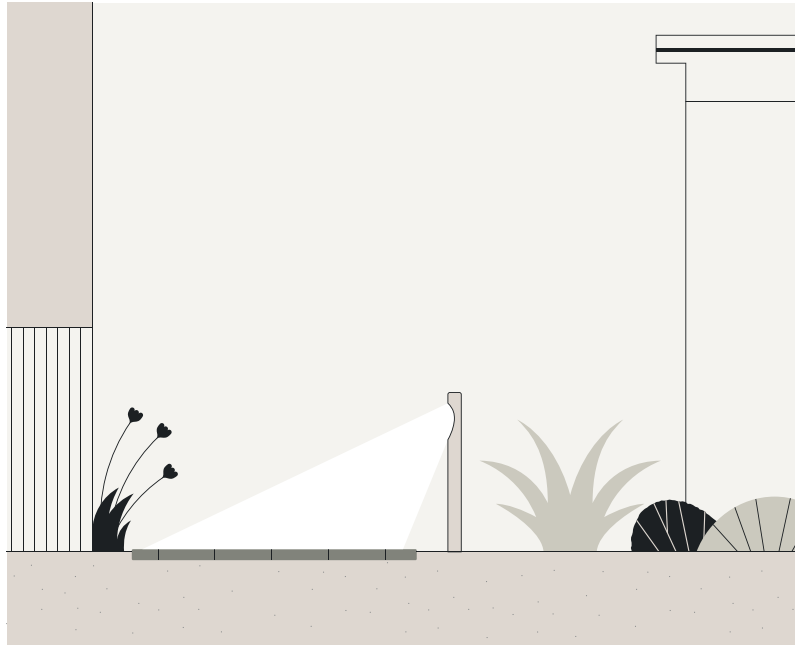
Lighting a path from a high bollard with asymmetrical lighting directs all the light to the path while the garden remains dark.
